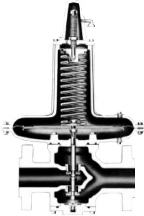
461-S with Double Seat Balanced Valve
