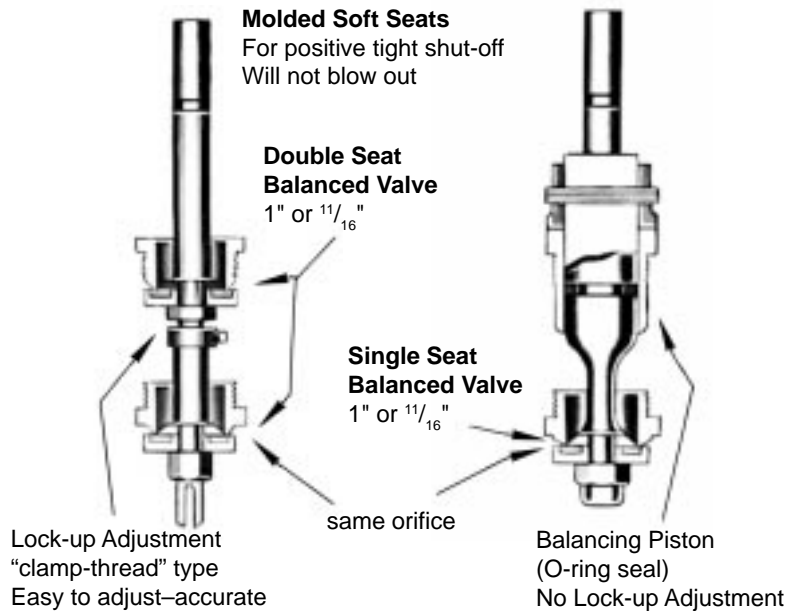
461-S with Single Seat Balanced Valve
