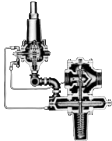
2" Model 1100 Pilot Operated Regulator See Bulletin R-1341
