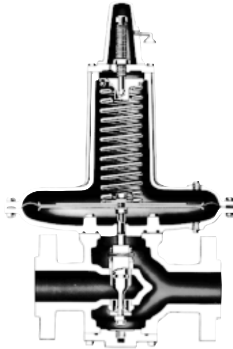
461-S with Single Seat Balanced Valve
