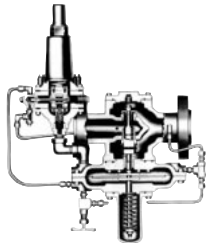
2" Model 1200 All steel construction Outlets to 600 psi See Bulletin R-1342
